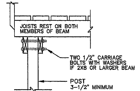
ALTERNATE BEAM (GOOD)
