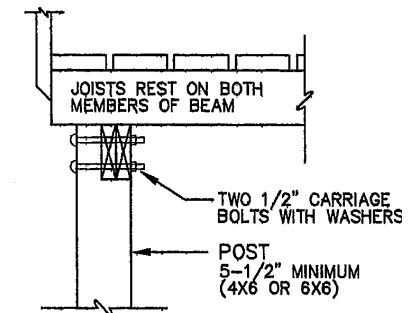
ALTERNATE BEAM (BETTER)
